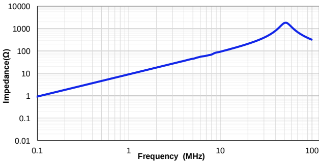
CSEB0420H-1R5M
